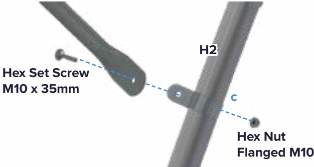
Attach lintel brace bar to hoop H2 .
